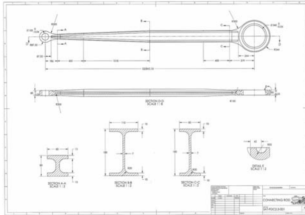
DETAILED ENGINEERING DRAWING OF A CONNECTING ROD FOR A STEAM LOCOMOTIVE, (IMAGE COURTESY OF DAVID WARDALE OF THE 5AT PROJECT)
