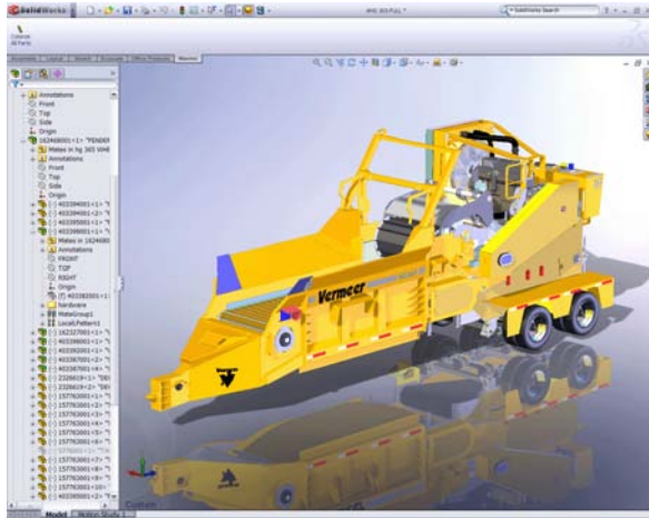
3D CAD MODEL OF A HORIZONTAL GRINDER (IMAGE COURTESY OF VERMEER ENVIRONMENTAL EQUIPMENT OF PELLA, IOWA)
